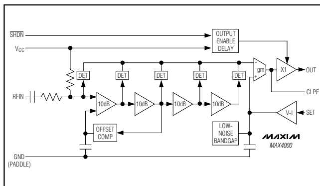
Figure 1. Functional Diagram
