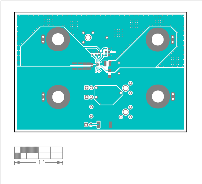
MAX38889A EV Kit PCB Layout—Top
