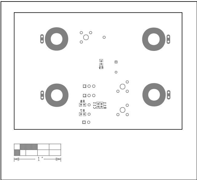
MAX38889A EV Kit Component Placement Guide—Bottom Silkscreen
