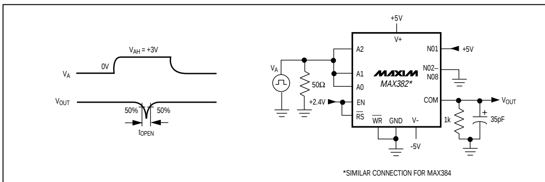
Figure 2. Break-Before-Make Interval ( t_{OPEN} )
