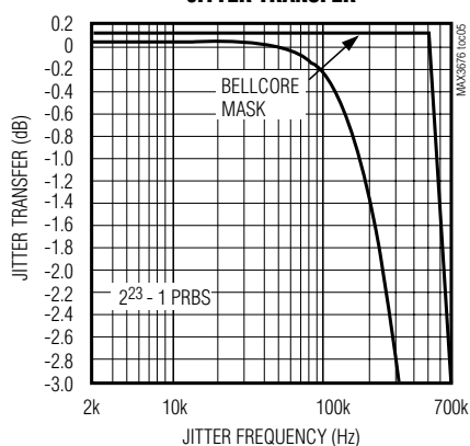
JITTER TRANSFER
