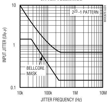
JITTER TOLERANCE
