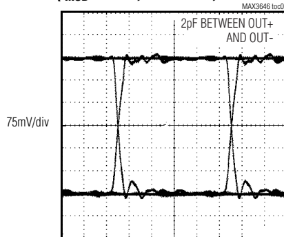
ELECTRICAL EYE DIAGRAM ( I_{MOD} = 30mA , 622.08MHz, 2 7 - 1 PRBS)
