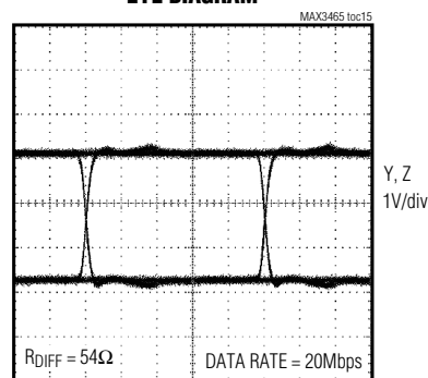
EYE DIAGRAM
