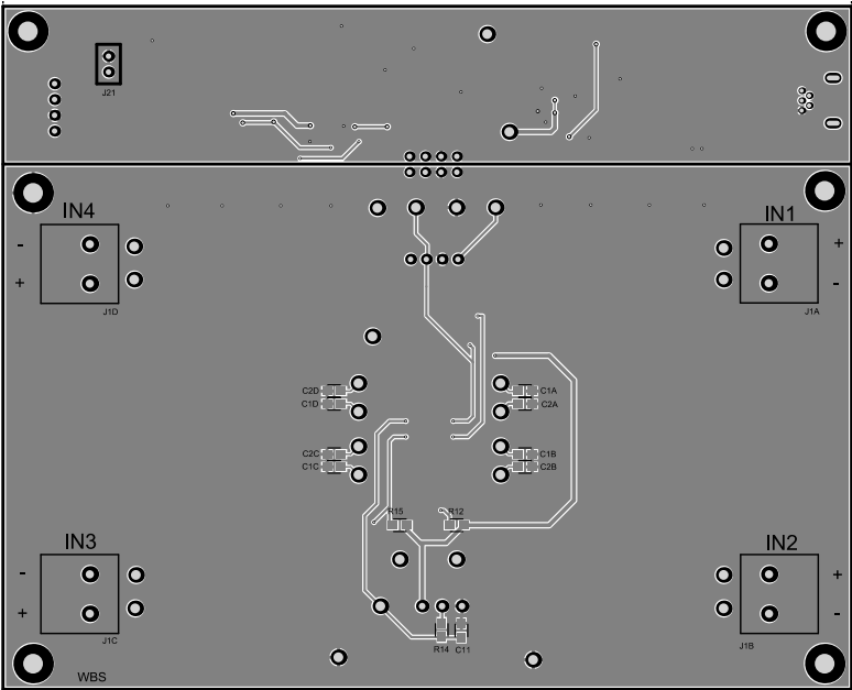
Figure 6. MAX34409 EV Kit PCB Layout—Bottom
