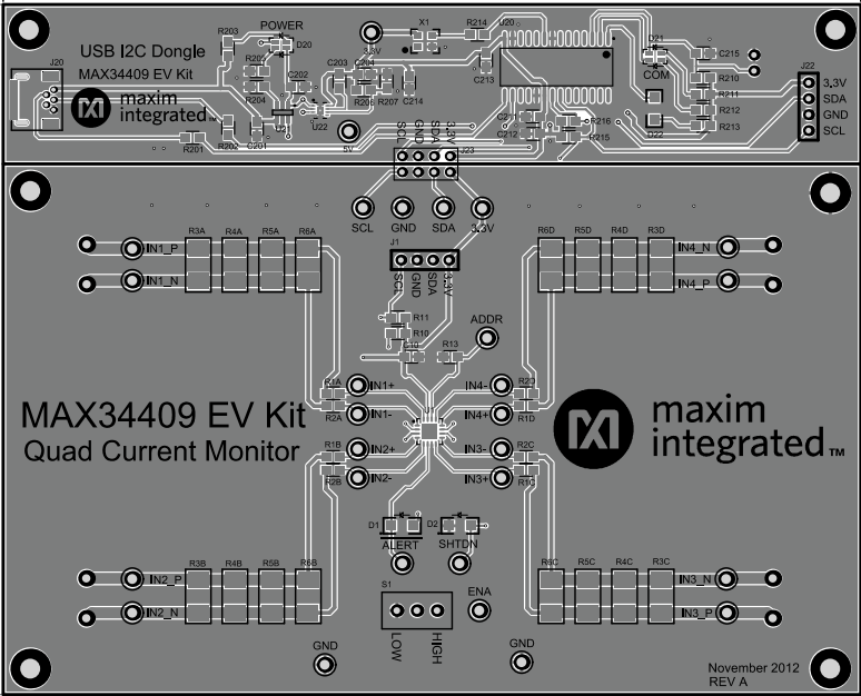
Figure 5. MAX34409 EV Kit PCB Layout—Top
