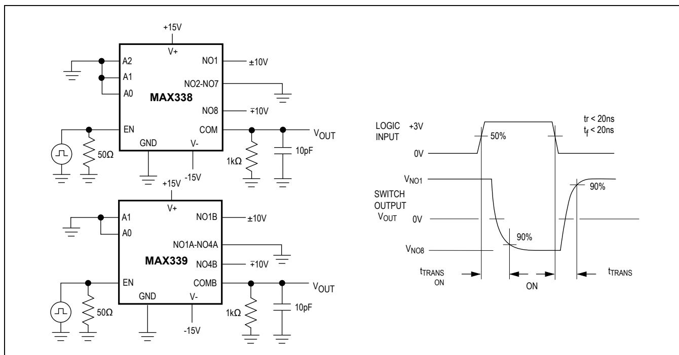
Figure 2. Transition Time
