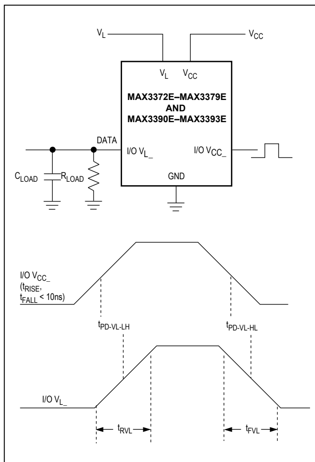
Figure 1b. Rail-to-Rail Driving I/O V_{CC}
