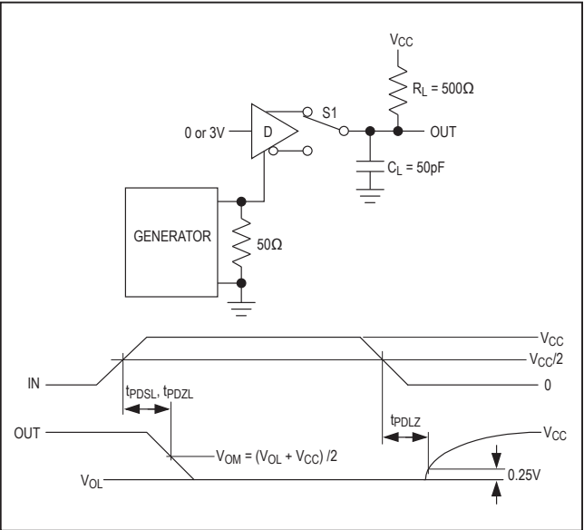
Figure 4. Driver Enable and Disable Times (tPDSL, tPDZL, tPDLZ, tPDZ)
