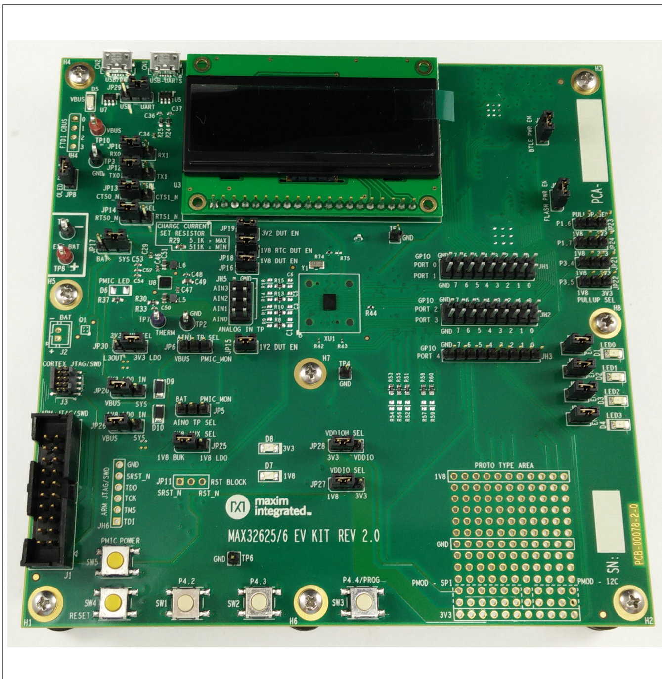
Figure 2. MAX32625 EV Kit Board
