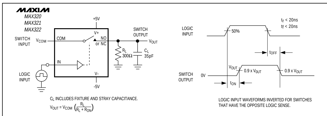
Figure 2. Switching Time
