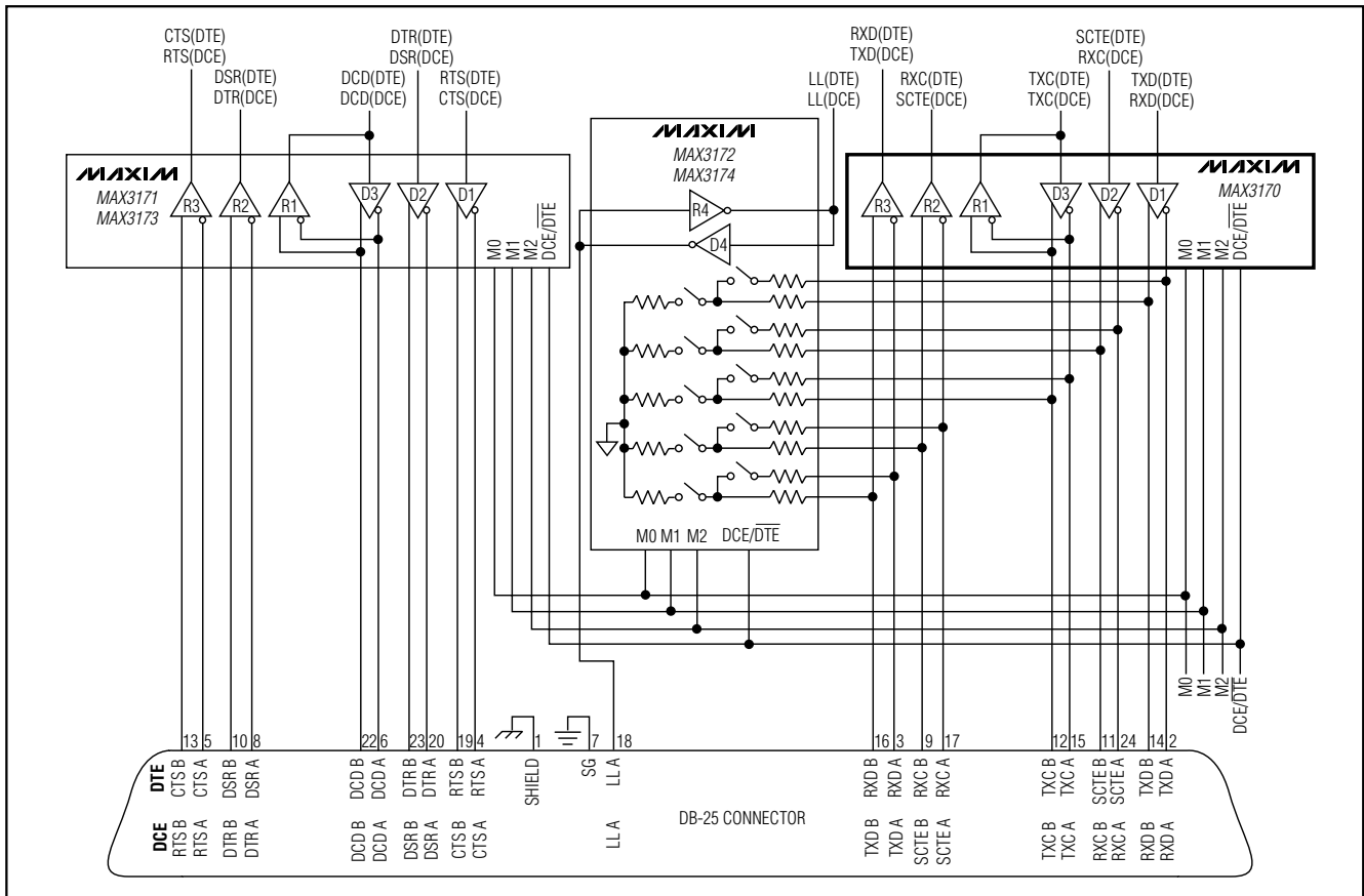
Figure 14. V.28 Termination and Internal Resistance Networks
