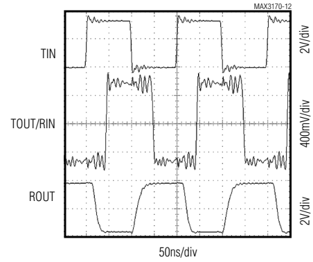
V.35 LOOPBACK SCOPE PHOTO
