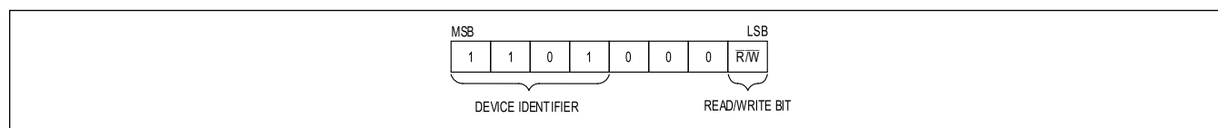
Figure 3. I 2 C Slave Address
