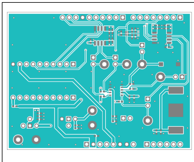
MAX31328 Shield PCB Layout—Top
