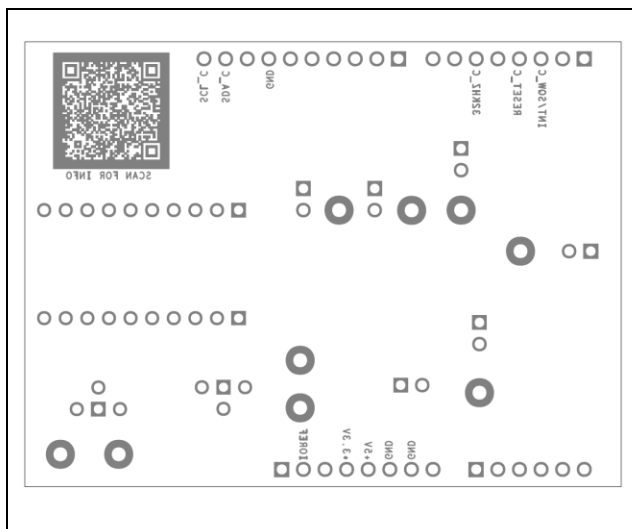
MAX31328 Shield PCB Layout— Bottom Silkscreen
