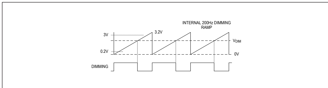
Figure 6. Analog-to-PWM Dimming
