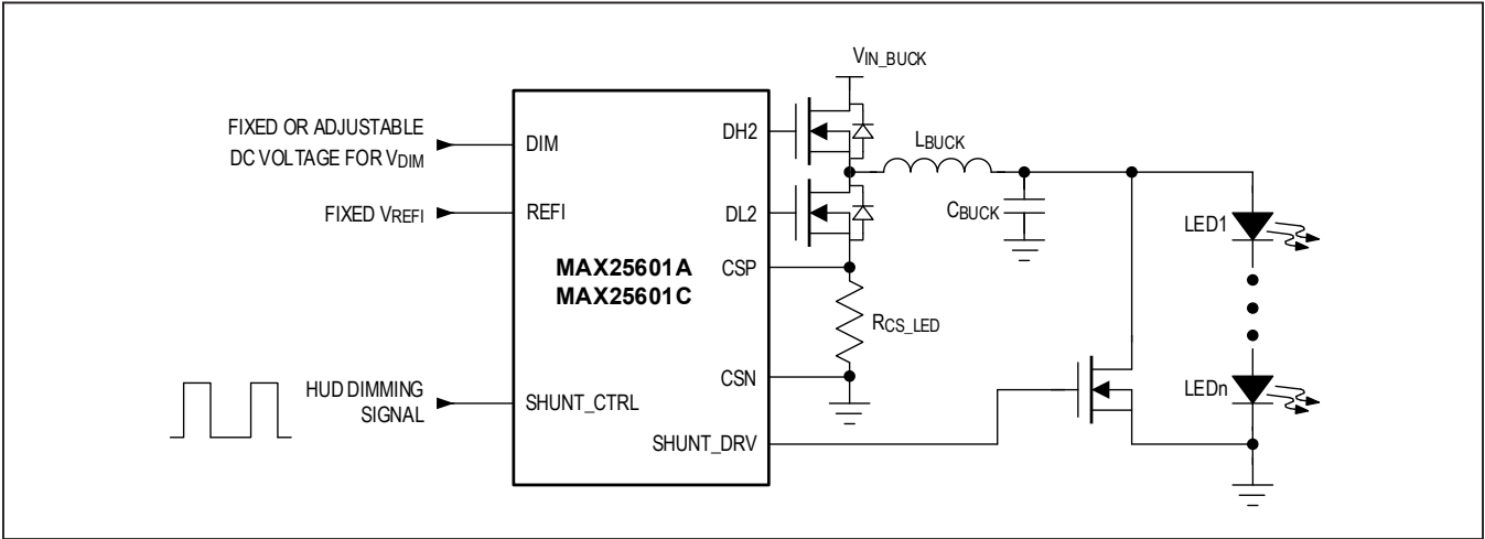
Figure 7. Shunt Dimming
