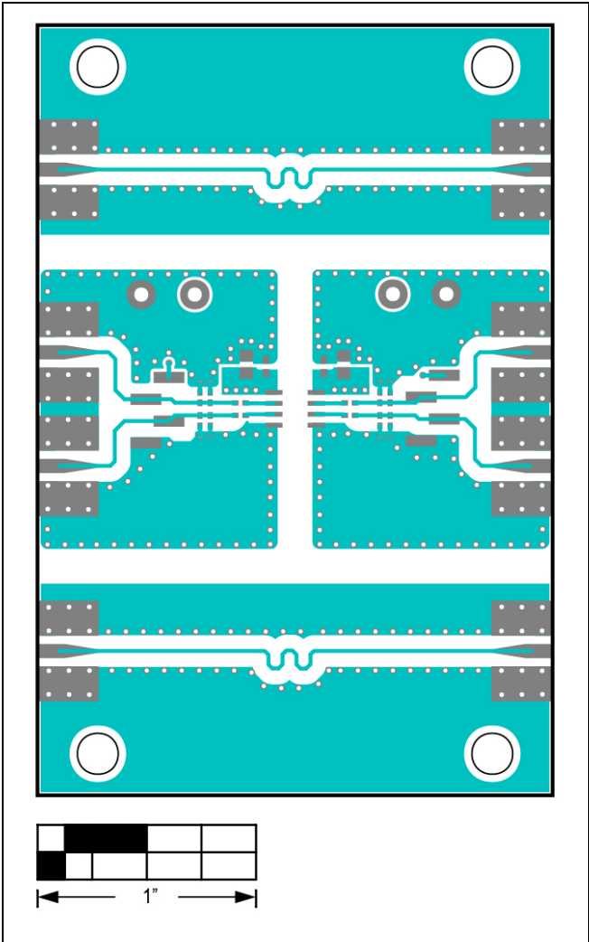
MAX22420/MAX22421 EV Kit PCB Layout—Top Layer
