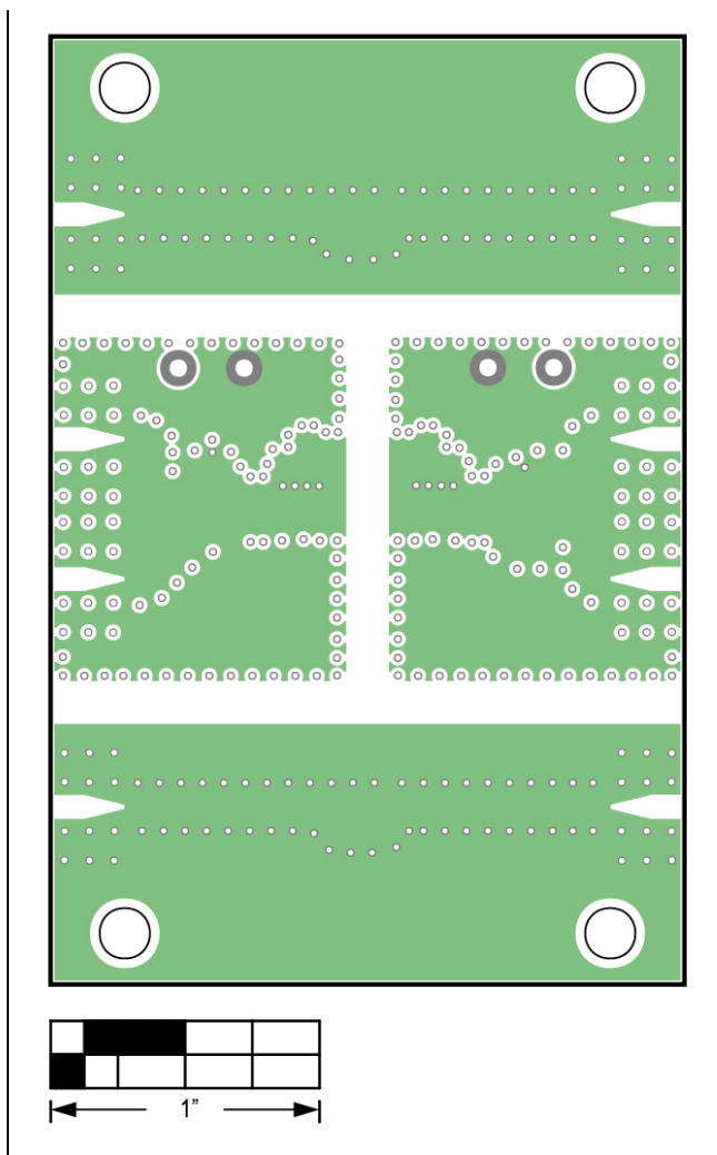
MAX22420/MAX22421 EV Kit PCB Layout—Layer 3 PWR
