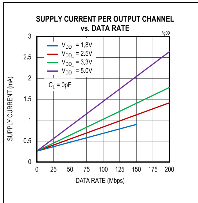
Figure 9. Supply Current per Output Channel (Estimated)
