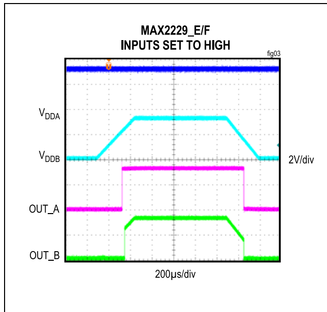
Figure 3. Undervoltage Lockout Behavior MAX2229_E/F Input High
