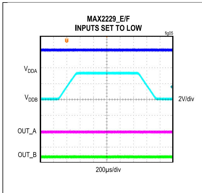
Figure 5. Undervoltage Lockout Behavior MAX2229_E/F Input Low
