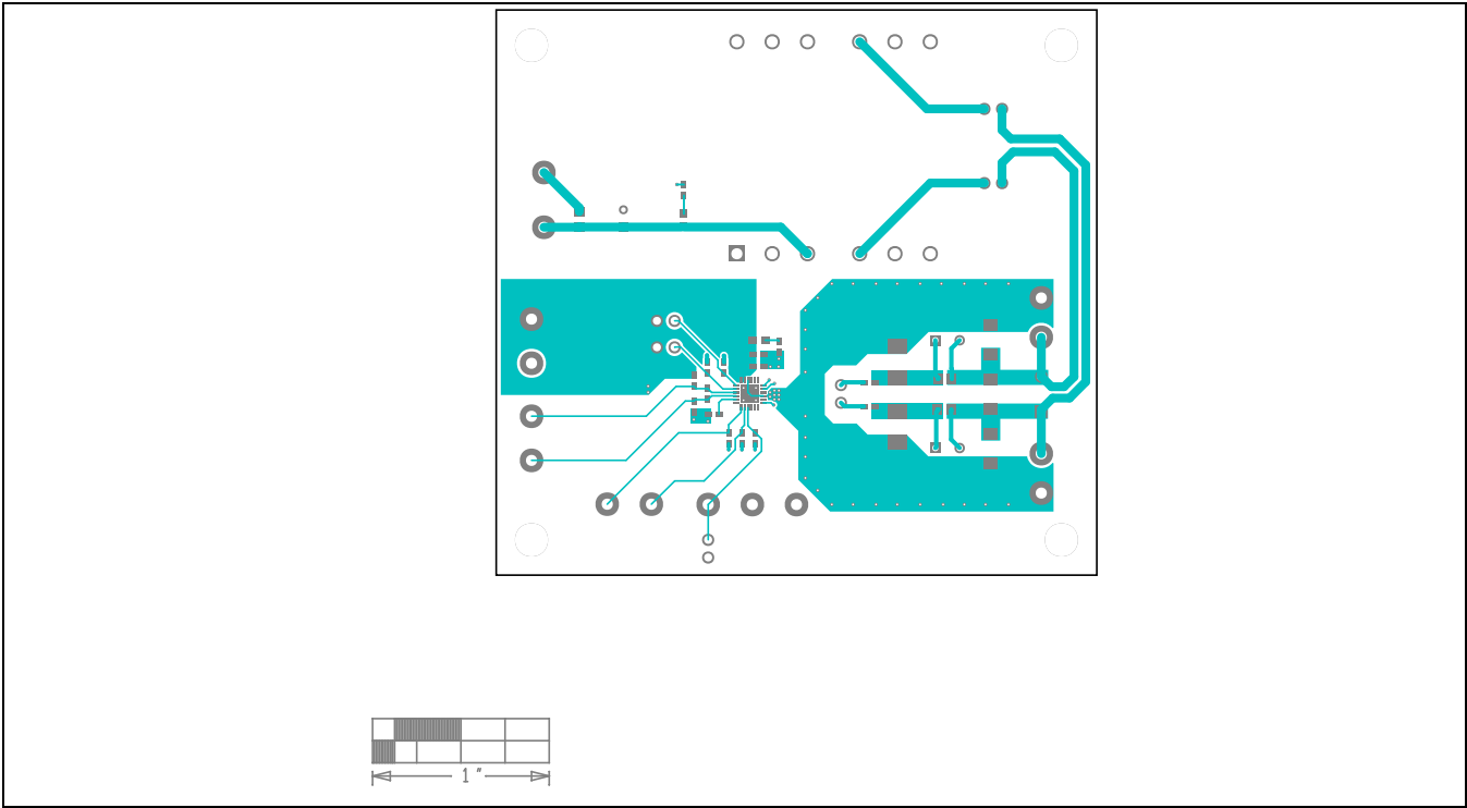
MAX22288 EV Kit PCB Layout—Top Layer
