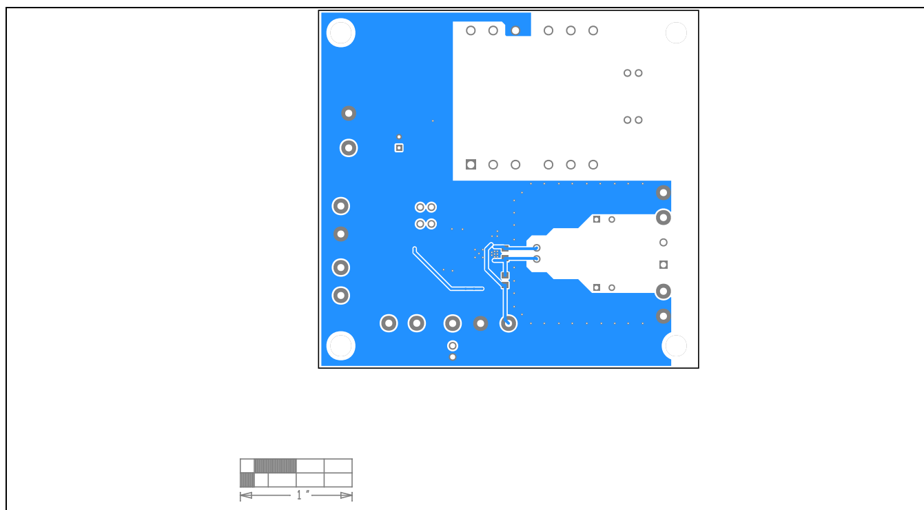
MAX22288 EV Kit PCB Layout—Bottom Layer
