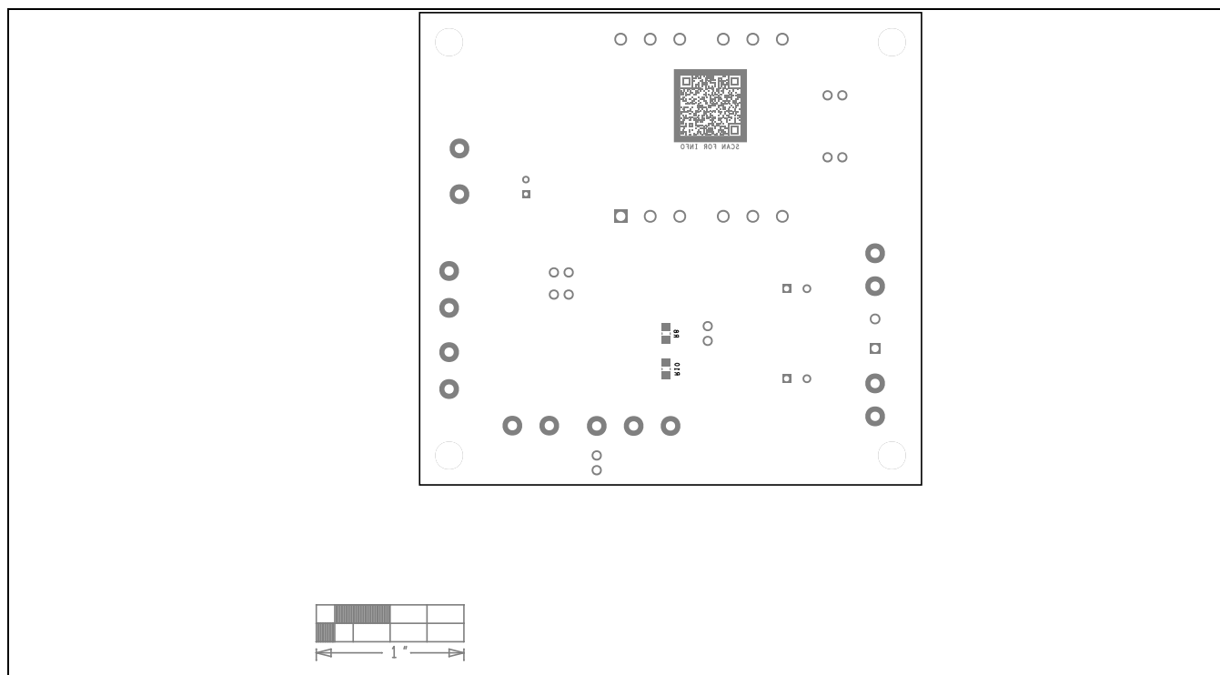
MAX22288 EV Kit PCB Layout—Bottom Silkscreen
