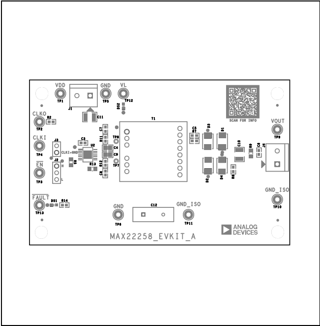
MAX22258 EV Kit PCB Layout—Top Silkscreen
