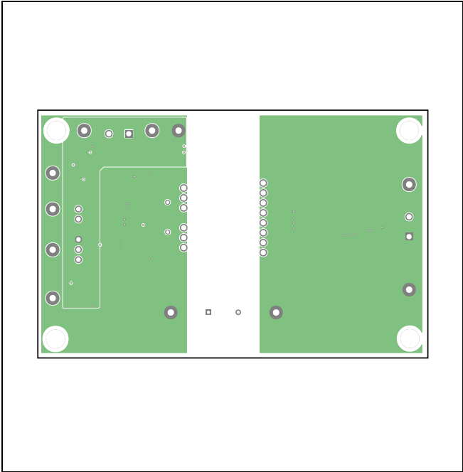
MAX22258 EV Kit PCB Layout—Layer 3
