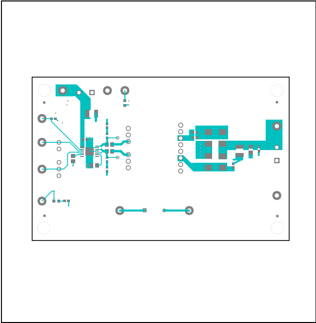
MAX22258 EV Kit PCB Layout—Top Layer
