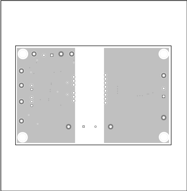
MAX22258 EV Kit PCB Layout—Layer 2
