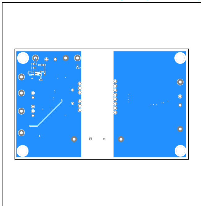
MAX22258 EV Kit PCB Layout—Bottom Layer
