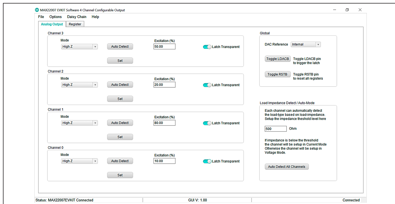
Figure 3. MAX22007 EV Kit Software, Load-Impedance Detect Setup
