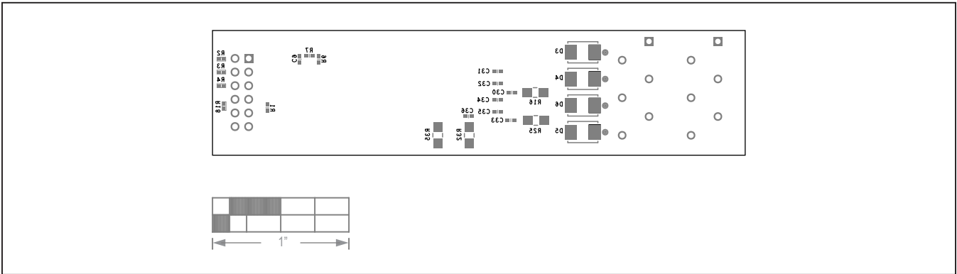
MAX22005PMB# PCB Layout—SILK_BOT
