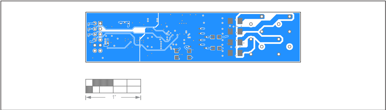
MAX22005PMB# PCB Layout—BOTTOM
