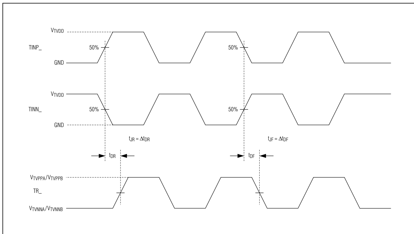
Figure 7. Jitter Timing
