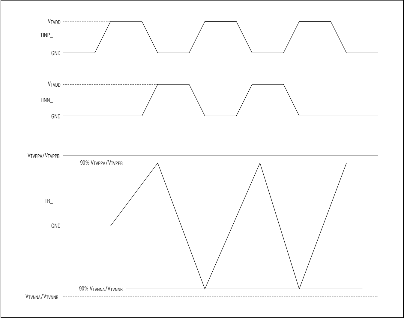
Figure 6. Bandwidth
