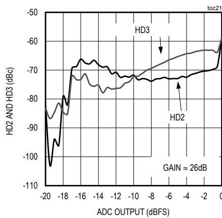
SECOND AND THIRD HARMONIC DISTORTION vs. ADC OUTPUT
