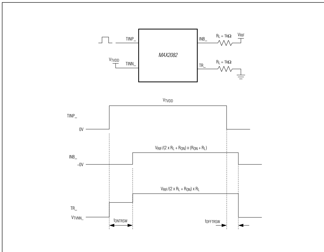
Figure 5. T/R Switch Turn-On/Off Time
