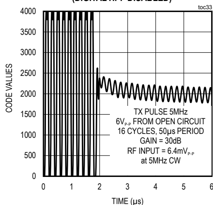
LNA OVERLOAD RECOVERY (DIGITAL HPF DISABLED)
