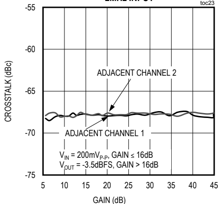
ADJACENT CHANNEL-TO-CHANNEL CROSSTALK vs. GAIN 2MHz INPUT
