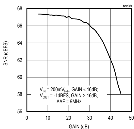
SNR vs. GAIN
