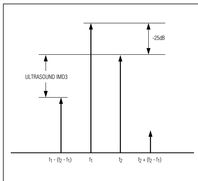
Figure 31. Ultrasound-Specific IMD3
