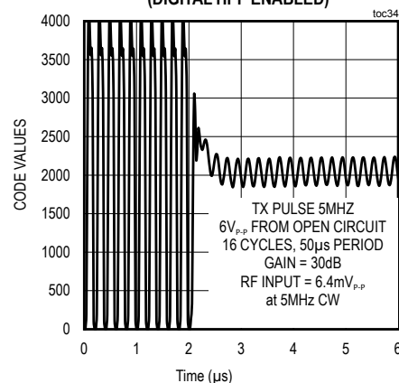
VGA OVERLOAD RECOVERY (DIGITAL HPF ENABLED)
