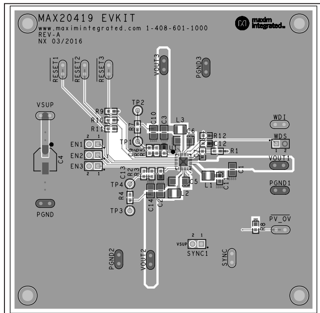
MAX20419 EV Kit Component Placement Guide---Top Layer
