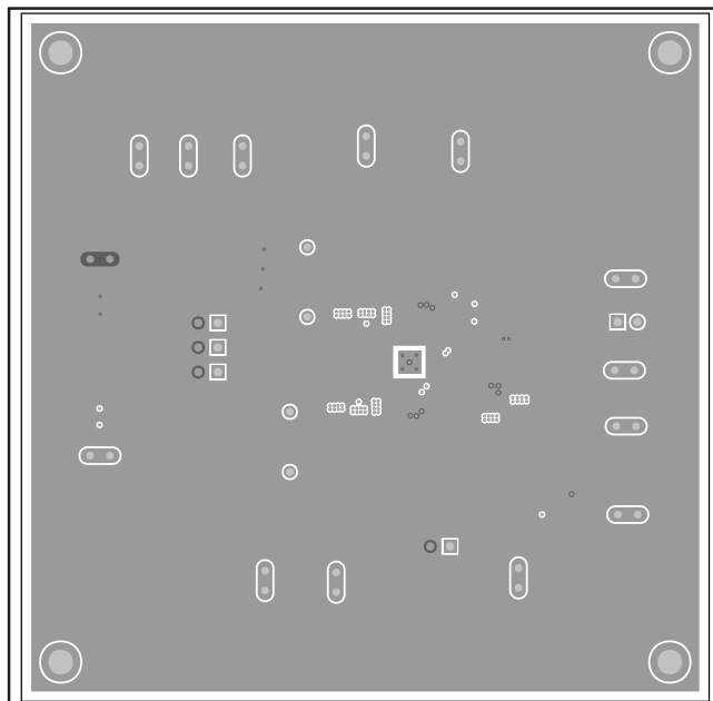
MAX20419 EV Kit PCB Layout---Layer 3 (ground layer)
