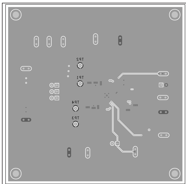
MAX20419 EV Kit Component Placement Guide---Bottom Layer
