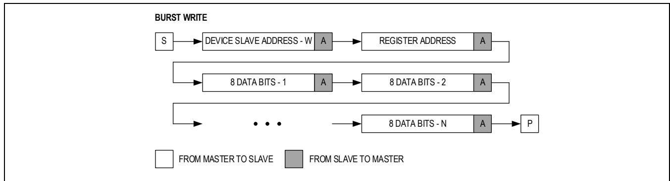
Figure 12. Burst Write Sequence
