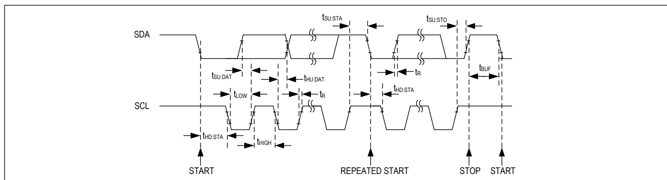
Figure 4. I²C Interface Timing
