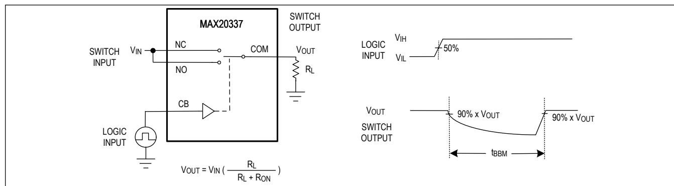
Figure 3. Break-Before-Make Interval
