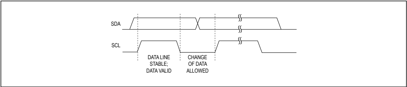
Figure 4. Bit Transfer
