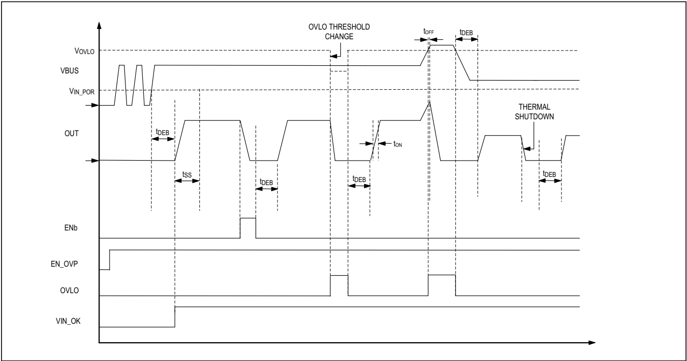
Figure 1. Timing Diagram
