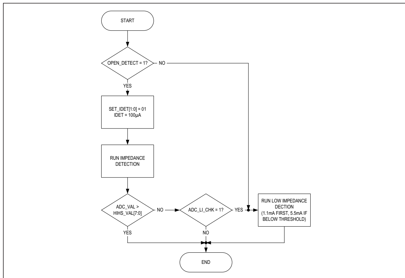
Figure 2. Impedance Detection Process
