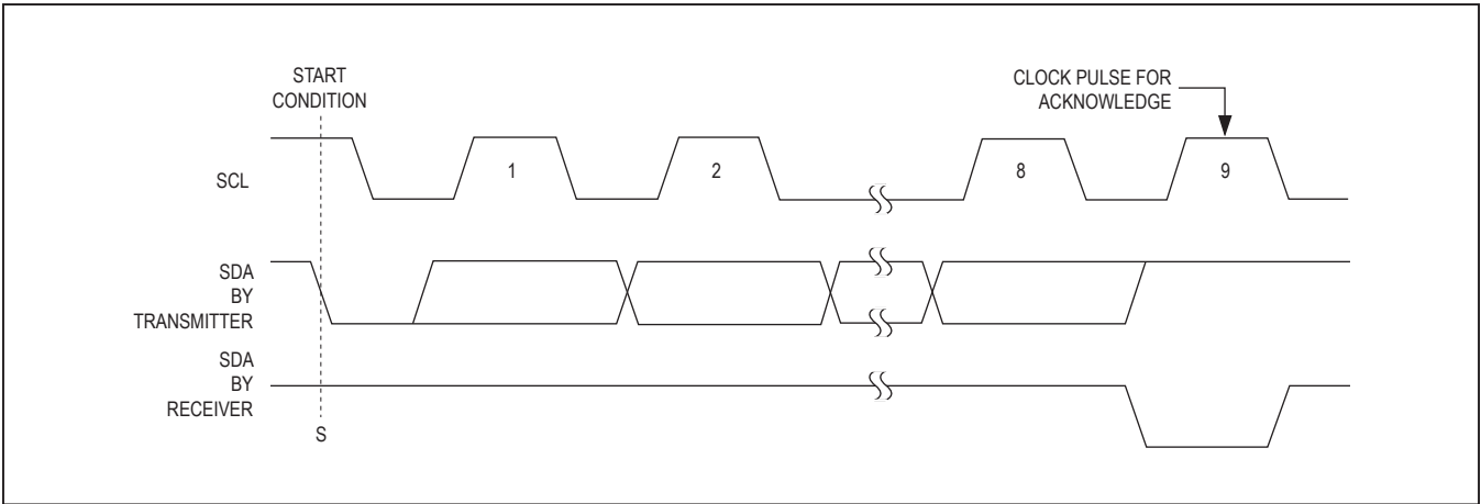
Figure 6. Acknowledge
