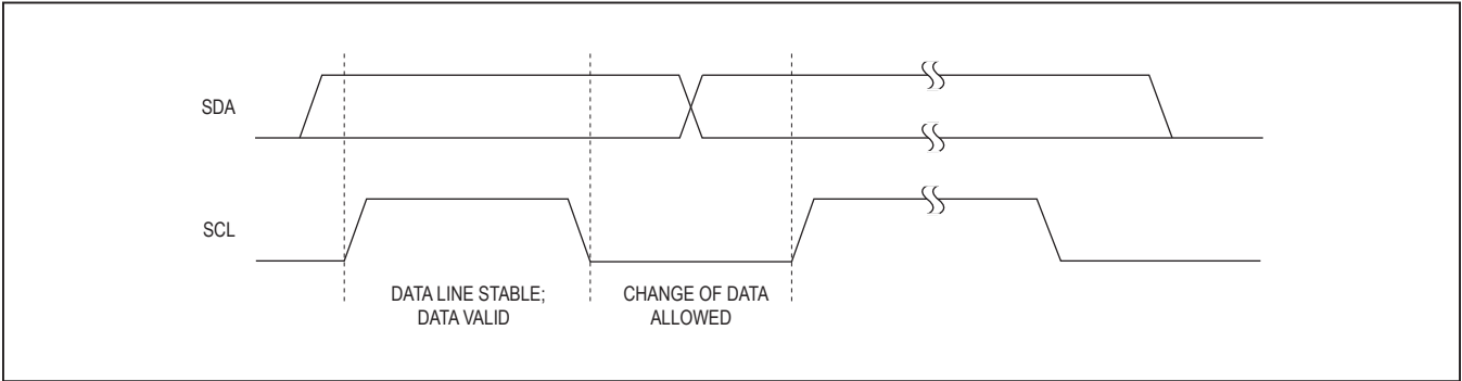
Figure 5. Bit Transfer
