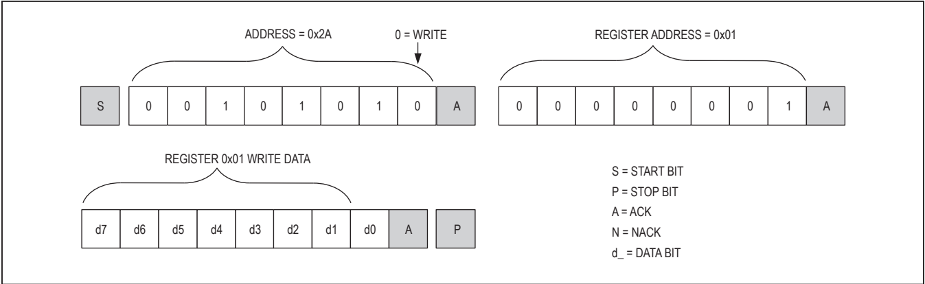
Figure 7. Format for I2C Write
