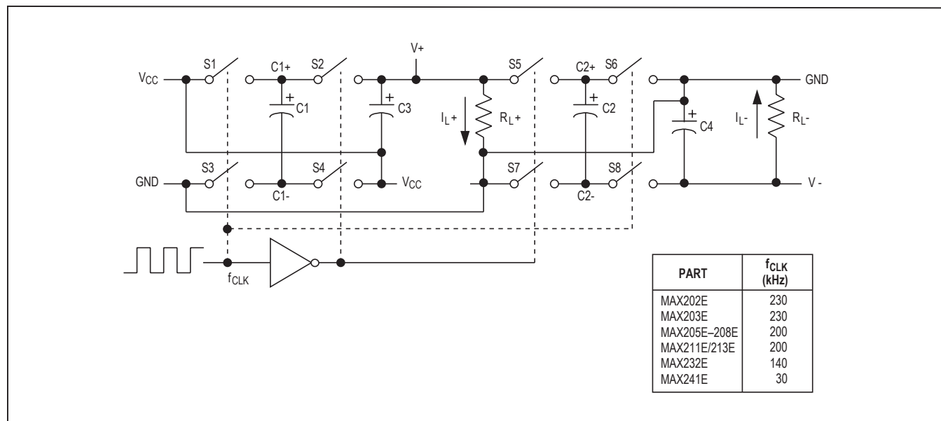
Figure 4. Charge-Pump Diagram
