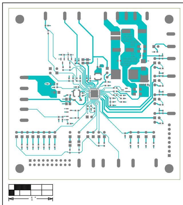
MAX20069 EV Kit PCB Layout—Top Layer
