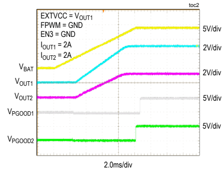
STARTUP INTO LOAD
