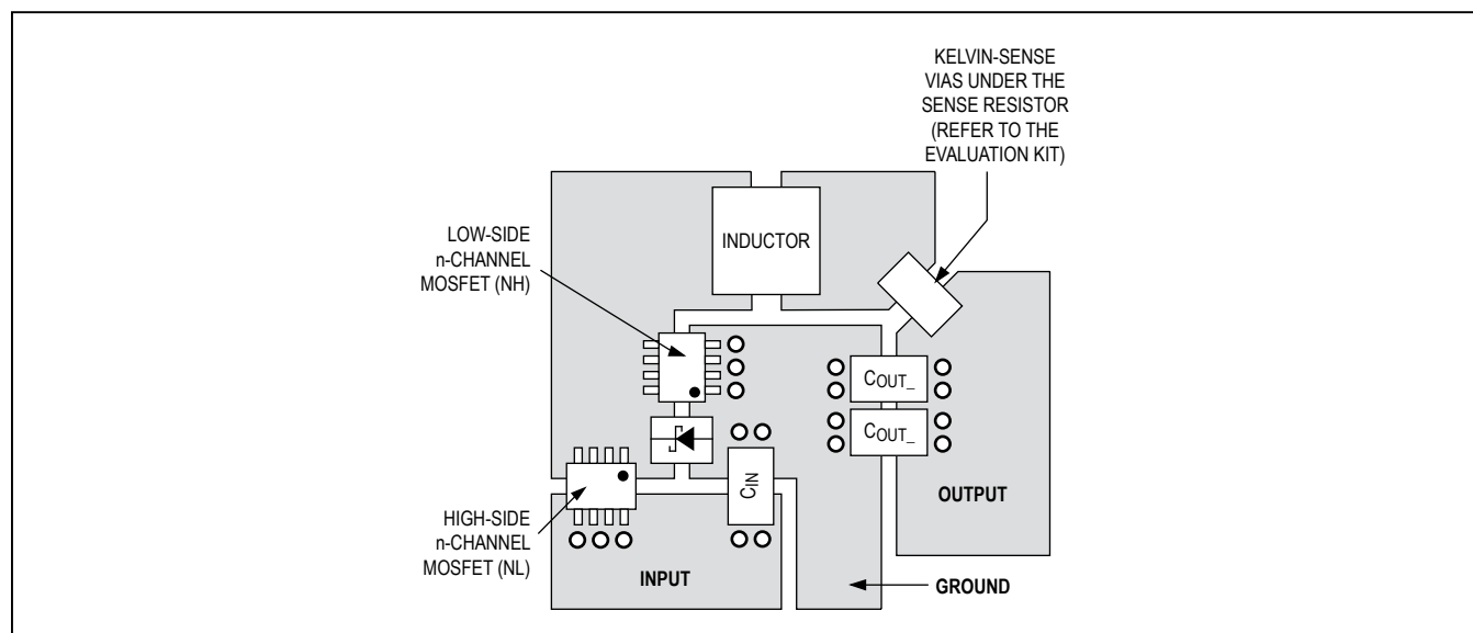
Figure 5. Layout Example
