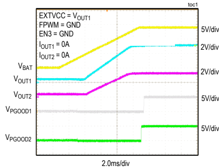
STARTUP INTO NO-LOAD
