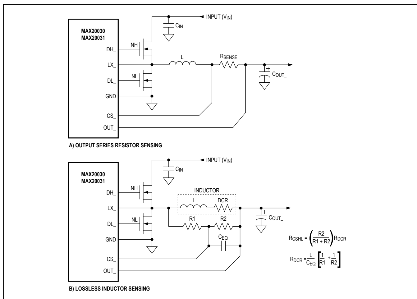
Figure 1. Current-Sense Configurations
