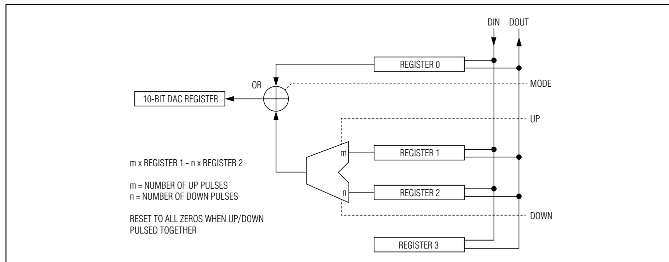
Figure 1. Register Configuration Diagram
