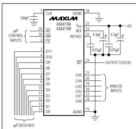
Figure 3. Operational Diagram
