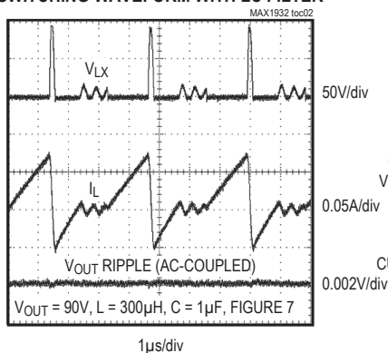
SWITCHING WAVEFORM WITH LC FILTER
