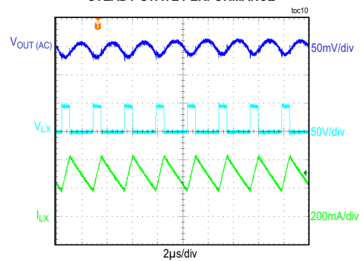
STEADY-STATE PERFORMANCE
