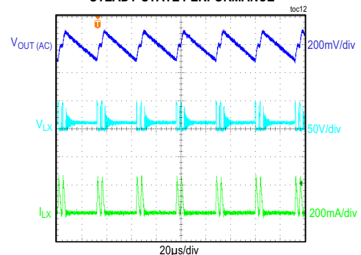
STEADY-STATE PERFORMANCE
