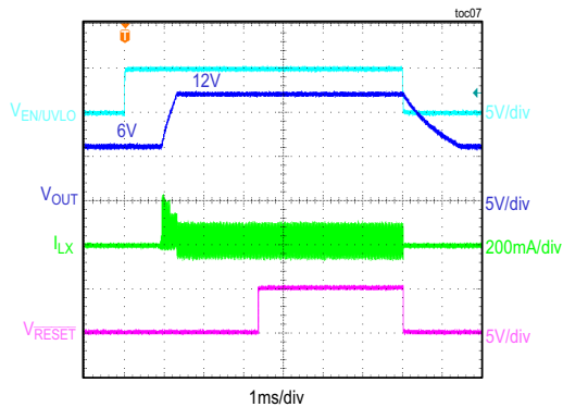
SOFT START WITH PREBIAS OF VOLTAGE OF 6V
