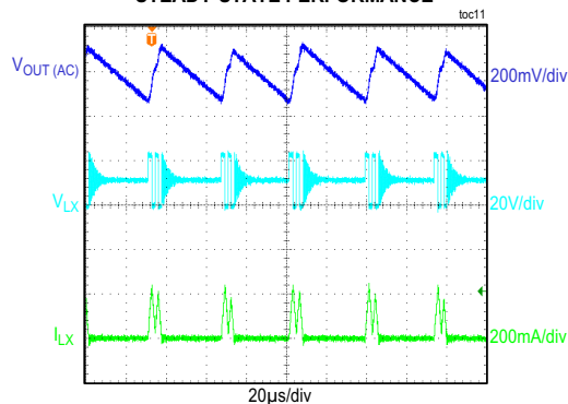
STEADY-STATE PERFORMANCE
