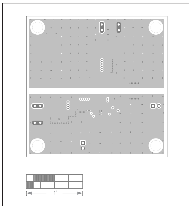
MAX17692BEVKIT# Layout—Layer 2
