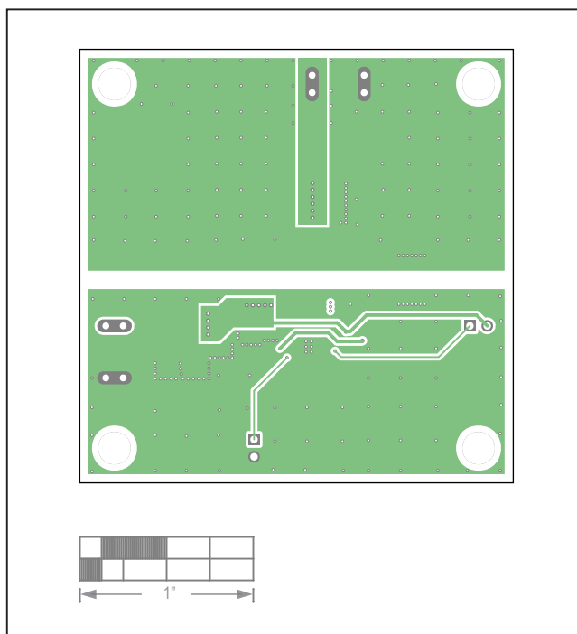
MAX17692BEVKIT# Layout—Layer 3
