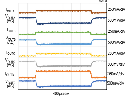
SECONDARY LOAD TRANSIENT RESPONSE (LOAD CURRENT STEPPED FROM 10% TO 100%)
