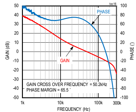
BODE PLOT
