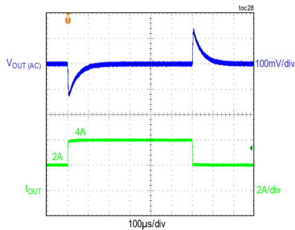
LOAD TRANSIENT BETWEEN 2A AND 4A FIGURE 4 AND FIGURE 6 CIRCUITS
