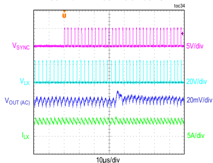
EXTERNAL CLOCK SYNCHRONIZATION FIGURE 3 AND FIGURE 5 CIRCUITS
