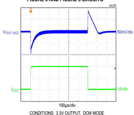
LOAD TRANSIENT BETWEEN 0.05A AND 2A FIGURE 3 AND FIGURE 5 CIRCUITS
