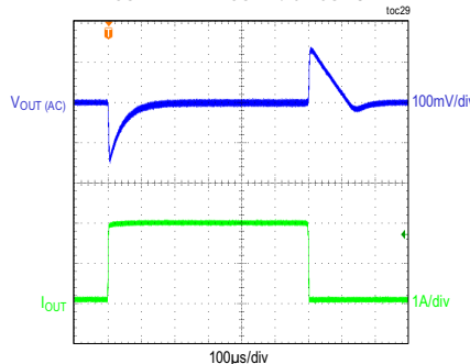
LOAD TRANSIENT BETWEEN 0.05A AND 2A FIGURE 4 AND FIGURE 6 CIRCUITS
