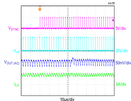
EXTERNAL CLOCK SYNCHRONIZATION FIGURE 4 AND FIGURE 6 CIRCUITS
