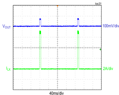
SHORT-CIRCUIT PROTECTION FIGURE 3 AND FIGURE 5 CIRCUITS
