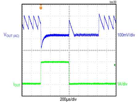
LOAD TRANSIENT BETWEEN 0.05A AND 2A FIGURE 4 AND FIGURE 6 CIRCUITS
