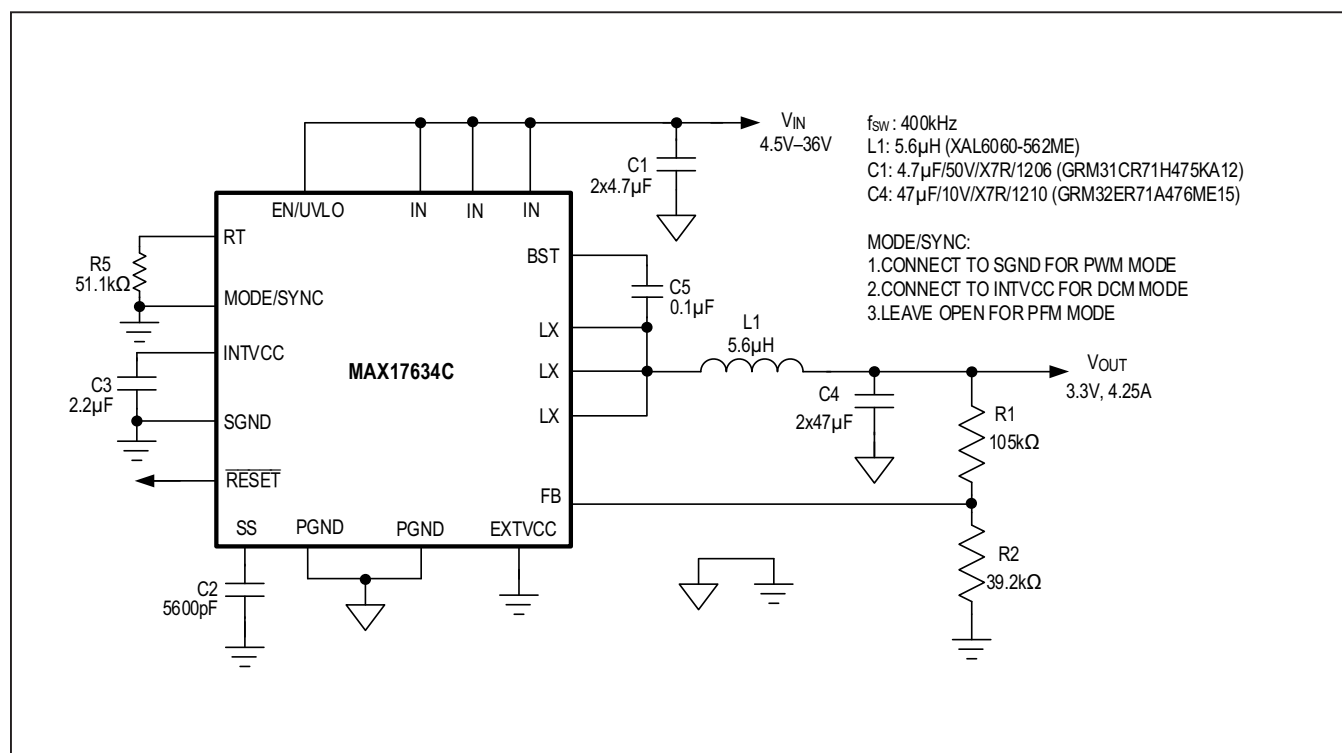
Figure 3. Adjustable 3.3V Output with 400kHz Switching Frequency
