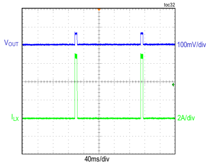
SHORT-CIRCUIT PROTECTION FIGURE 4 AND FIGURE 6 CIRCUITS
