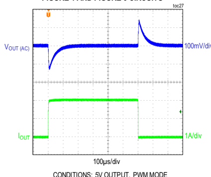
LOAD TRANSIENT BETWEEN 0A AND 2A FIGURE 4 AND FIGURE 6 CIRCUITS
