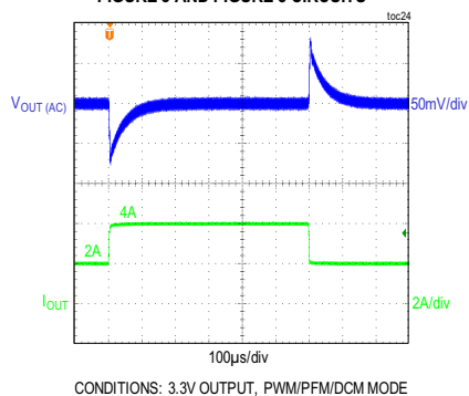
LOAD TRANSIENT BETWEEN 2A AND 4A FIGURE 3 AND FIGURE 5 CIRCUITS
