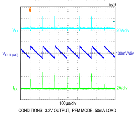
STEADY-STATE PERFORMANCE FIGURE 3 AND FIGURE 5 CIRCUITS
