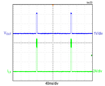
OVERLOAD PROTECTION FIGURE 4 AND FIGURE 6 CIRCUITS
