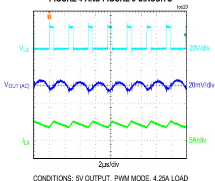
STEADY-STATE PERFORMANCE FIGURE 4 AND FIGURE 6 CIRCUITS
