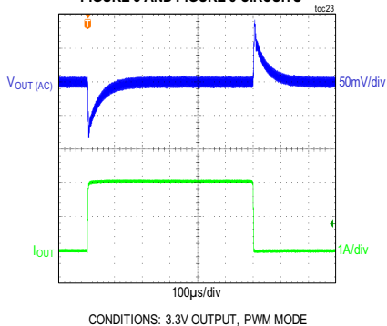
LOAD TRANSIENT BETWEEN 0A AND 2A FIGURE 3 AND FIGURE 5 CIRCUITS
