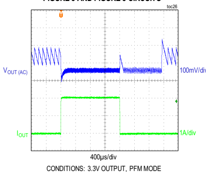
LOAD TRANSIENT BETWEEN 0.05A AND 2A FIGURE 3 AND FIGURE 5 CIRCUITS
