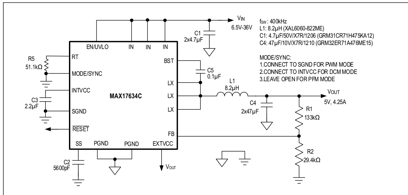
Figure 4. Adjustable 5V Output with 400kHz Switching Frequency
