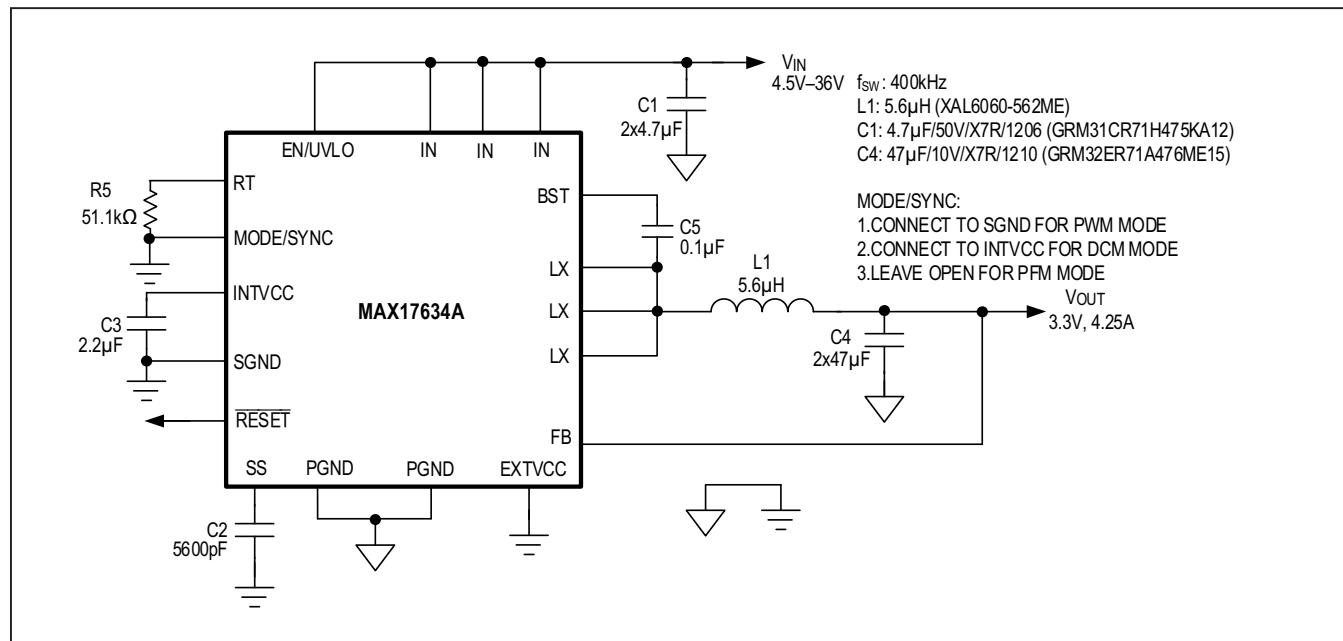
Figure 5. Fixed 3.3V Output with 400kHz Switching Frequency
