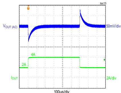
LOAD TRANSIENT BETWEEN 2A AND 4A
