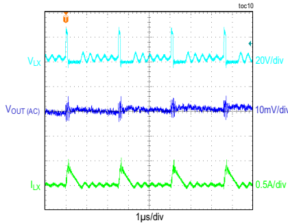
STEADY-STATE PERFORMANCE
