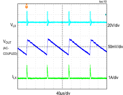
STEADY-STATE PERFORMANCE
