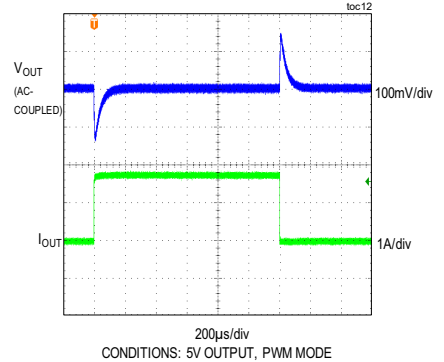
LOAD TRANSIENT BETWEEN 0A AND 1.75A
