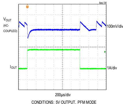
LOAD TRANSIENT BETWEEN 0A AND 1.75A
