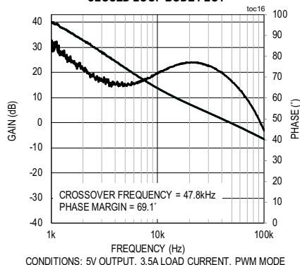
CLOSED LOOP BODE PLOT
