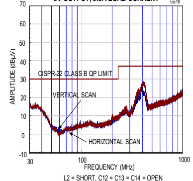
RADIATED EMI CURVE 5V OUTPUT, 3.5A LOAD CURRENT
