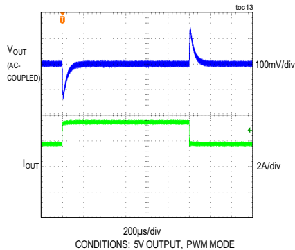
LOAD TRANSIENT BETWEEN 1.75A AND 3.5A
