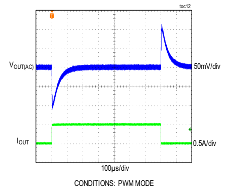
LOAD TRANSIENT RESPONSE BETWEEN 0A AND 0.5A
