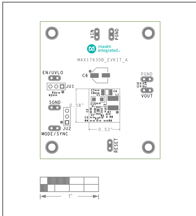
MAX17630BEVKIT# EV Kit—Top Silkscreen
