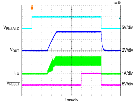
SOFT-START/SHUTDOWN THROUGH EN/UVLO
