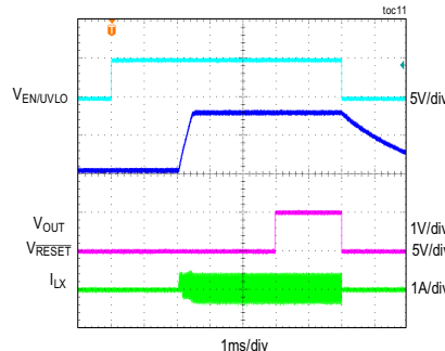
SOFT-START WITH PREBIAS VOLTAGE OF 1.65V
