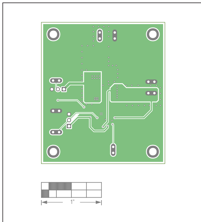
MAX17630AEVKIT# EV Kit—Layer 3
