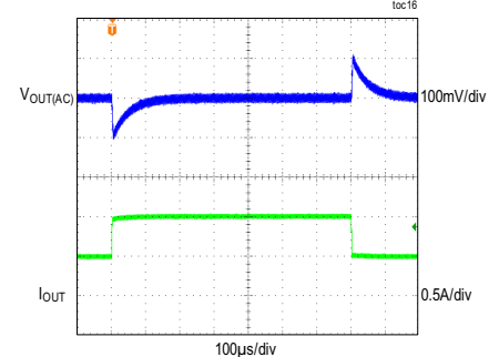
LOAD TRANSIENT RESPONSE BETWEEN 0.5A AND 1A
