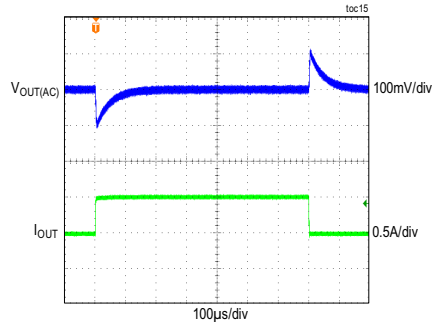
LOAD TRANSIENT RESPONSE BETWEEN 0A AND 0.5A
