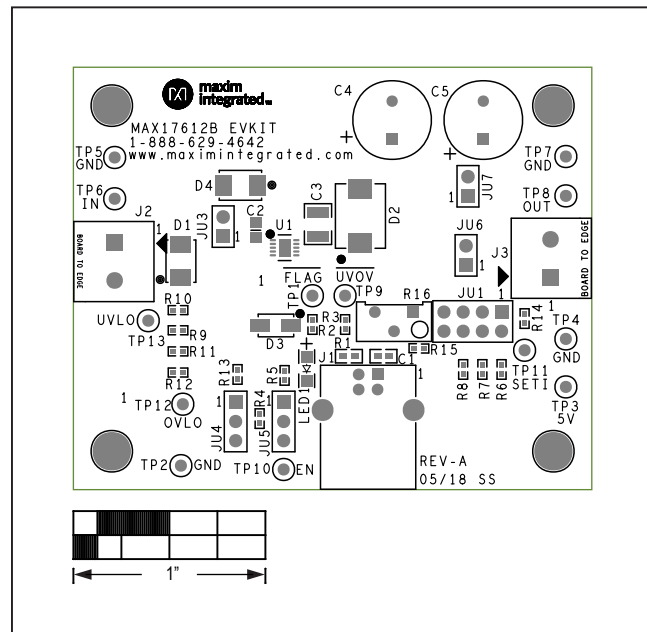
MAX17612B EV Kit PCB Layout—Top Silkscreen
