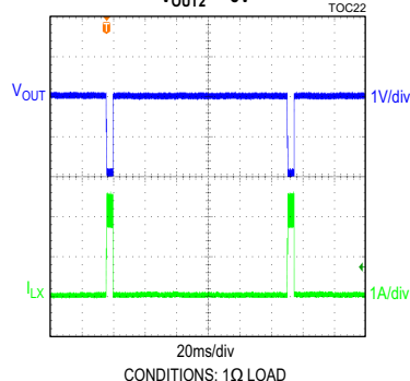
MAX17578 OVERLOAD PROTECTION VOUT2 = -5V
