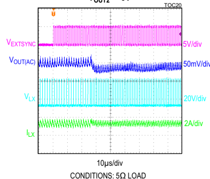
MAX17578 EXTERNAL CLOCK SYNCHRONIZATION WITH 840kHz VOUT2 = -5V
