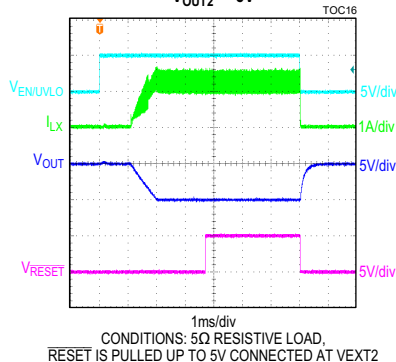
MAX17578 START UP & SHUT DOWN THROUGH EN/UVLO VOUT2 = -5V
