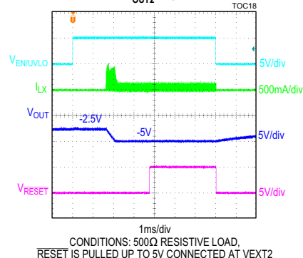
MAX17578 START UP WITH PREBIAS VOLTAGE OF -2.5V VOUT2 = -5V
