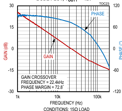
MAX17577 BODE PLOT, VOUT1 = -12V
