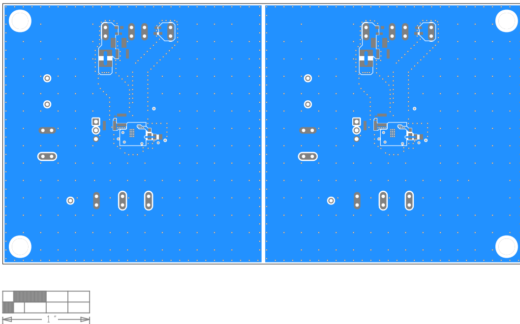
MAX17577EVKIT# and MAX17578EVKIT# EV Kits PCB Layout—Bottom Layer
