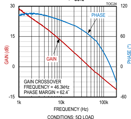
MAX17578 BODE PLOT, VOUT2 = -5V
