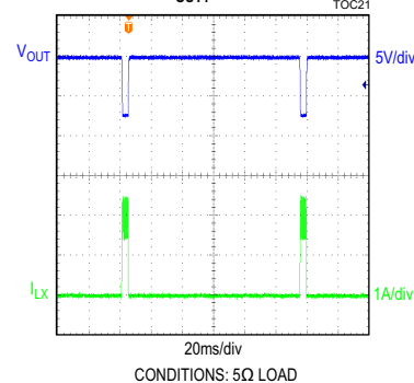
MAX17577 OVERLOAD PROTECTION VOUT1 = -12V
