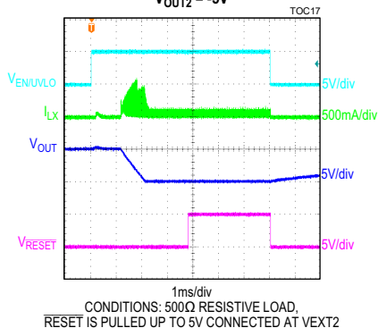
MAX17578 START UP & SHUT DOWN THROUGH EN/UVLO VOUT2 = -5V
