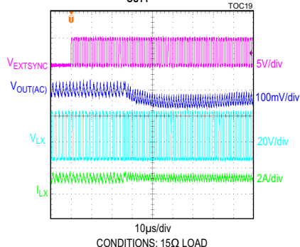
MAX17577 EXTERNAL CLOCK SYNCHRONIZATION WITH 840kHz VOUT1 = -12V
