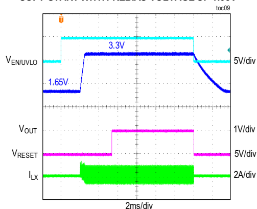
SOFT-START WITH PREBIAS VOLTAGE OF 1.65V
