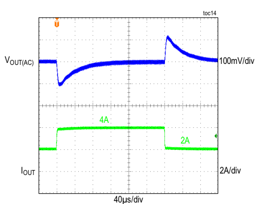
LOAD TRANSIENT BETWEEN 2A AND 4A
