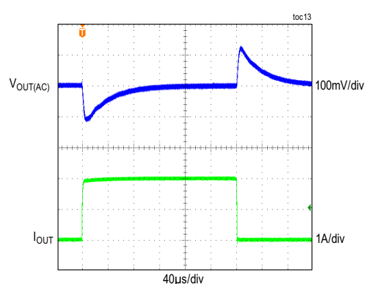
LOAD TRANSIENT BETWEEN 0A AND 2A
