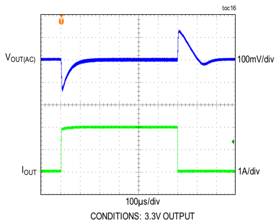
LOAD TRANSIENT BETWEEN 80mA AND 2A
