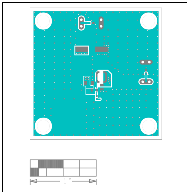
MAX17554B EV Kit PCB Layout—Top
