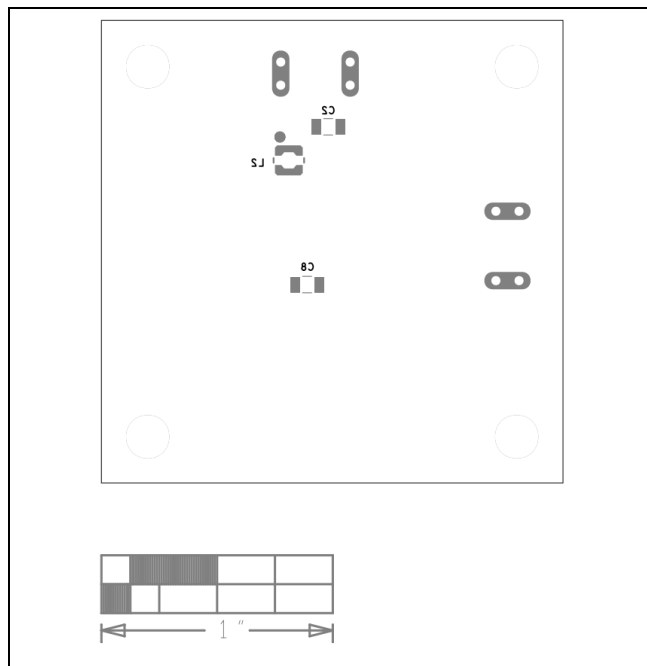
MAX17554B EV Kit Component Placement Guide—Bottom Silkscreen
