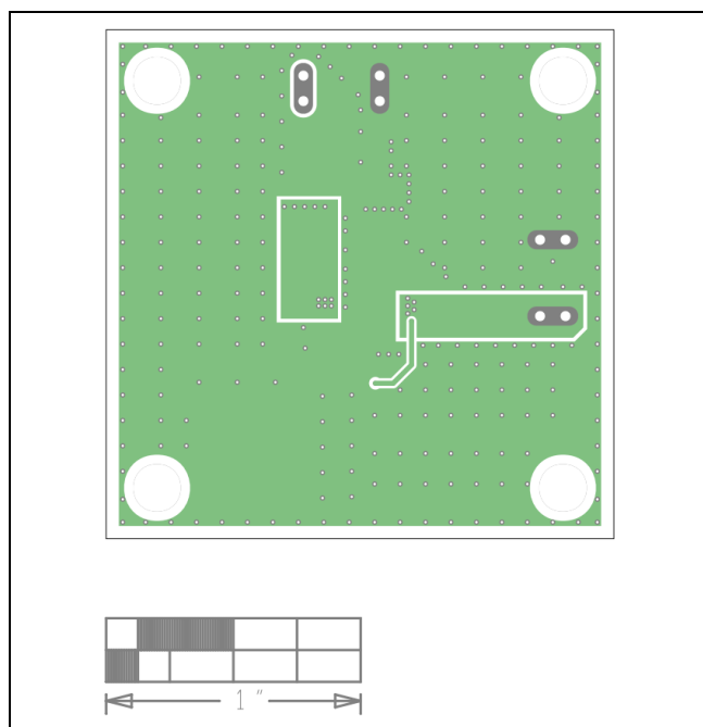
MAX17554B EV Kit PCB Layout—Layer 3
